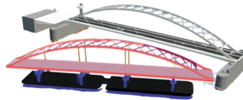
2) WBBb lift-off
