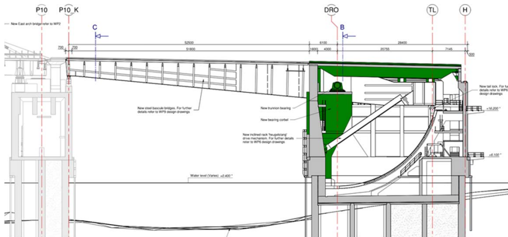
Bascule Bridges – Future situation
