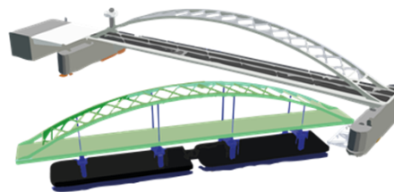
3) WBBn lift-in
