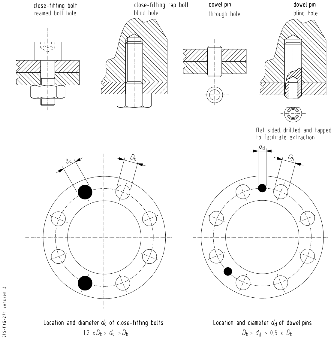
Figure 12: Close-fitting bolts and dowel pins
