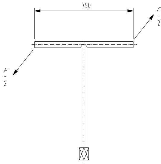
Gasunie standard T-Wrench for surface box operation
