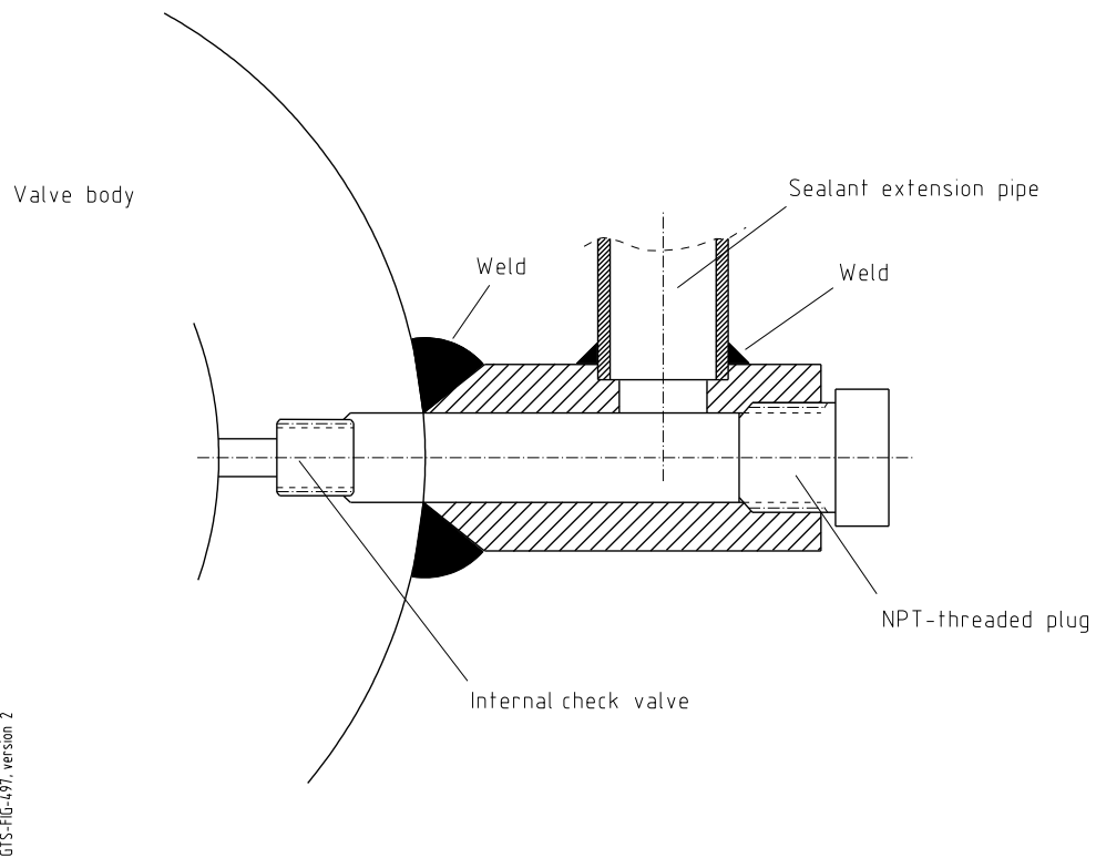
Figure 16: Details of seat sealant injection connection for underground valves
