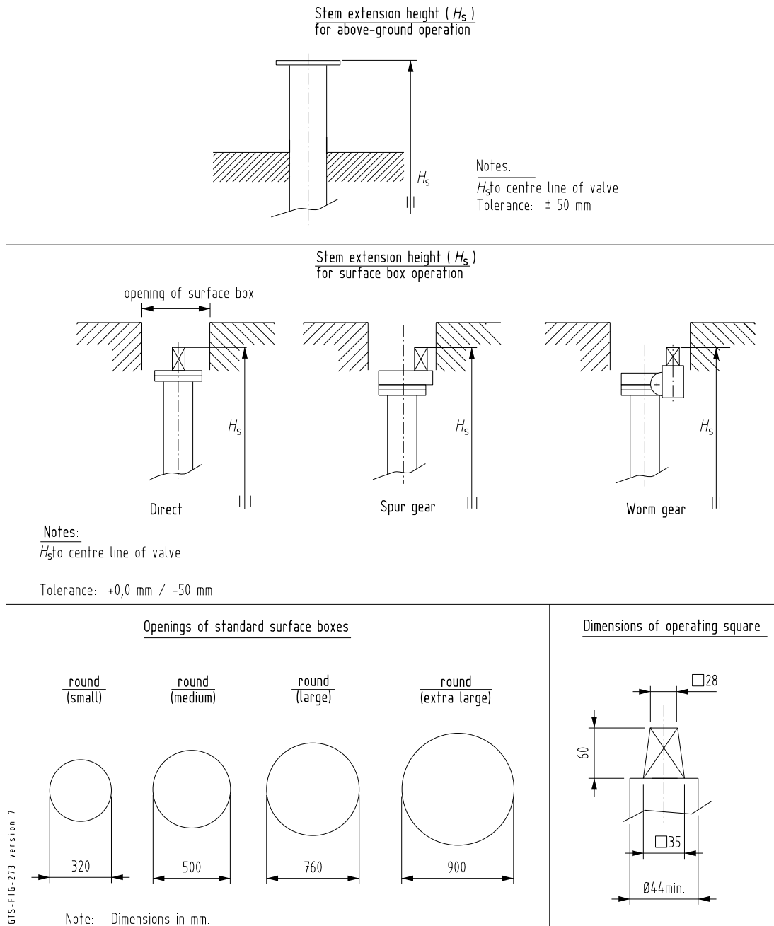
Figure 11: Stem extension height, surface box openings and operating square
