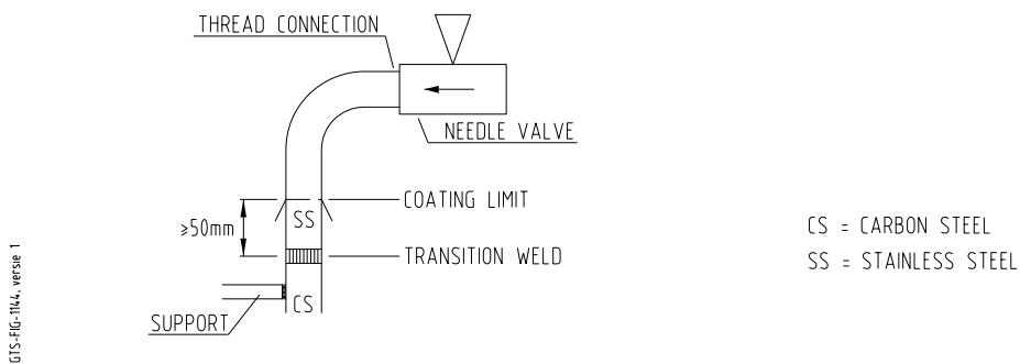
Figure 9: Aboveground configuration
