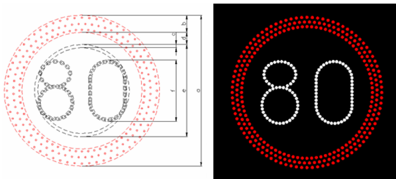
Figure M.2 — Example for calculation of dimensions of circular mandatory VMS
