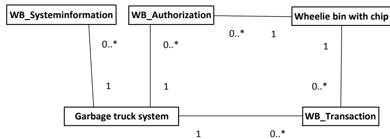
Figure 5: Domain model
