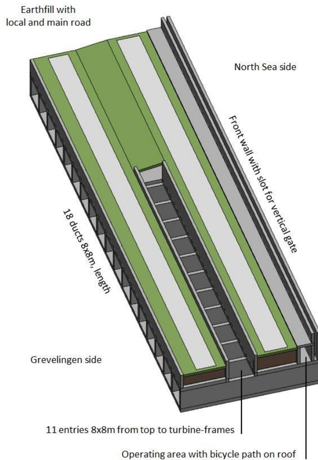
Figure 9: The structure of a flood barrier with tidal power plant in the location filled in with soil.
