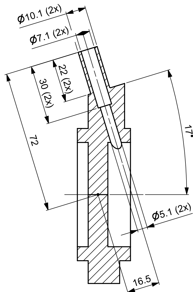
SECTION B-B
