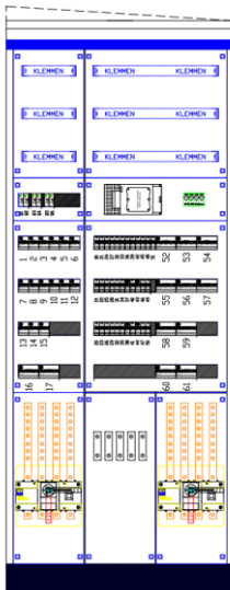
Verdeelkast OVK-0.1 hxbxd 2000x800x450mm IP 54
